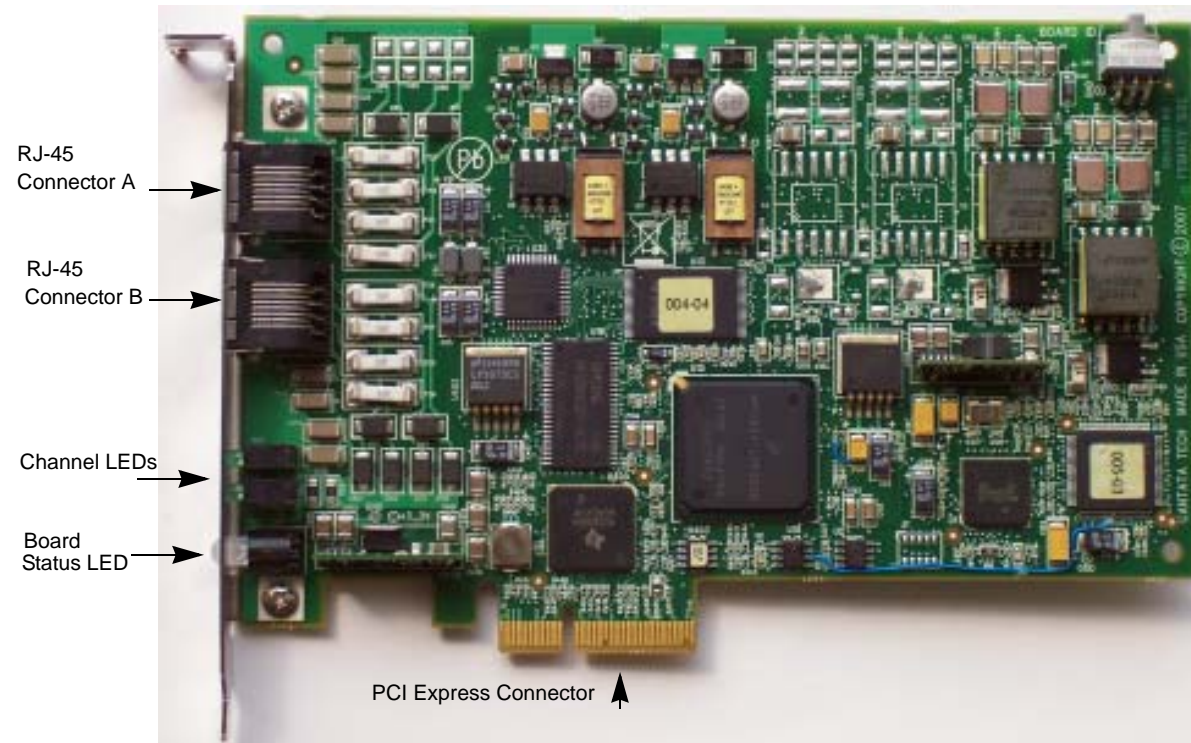
Figure 4. Dialogic® Brooktrout® TR1034 DID, Combo & Loop Start PCI Express Board
