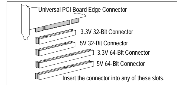
Figure 3. PCI Slots
