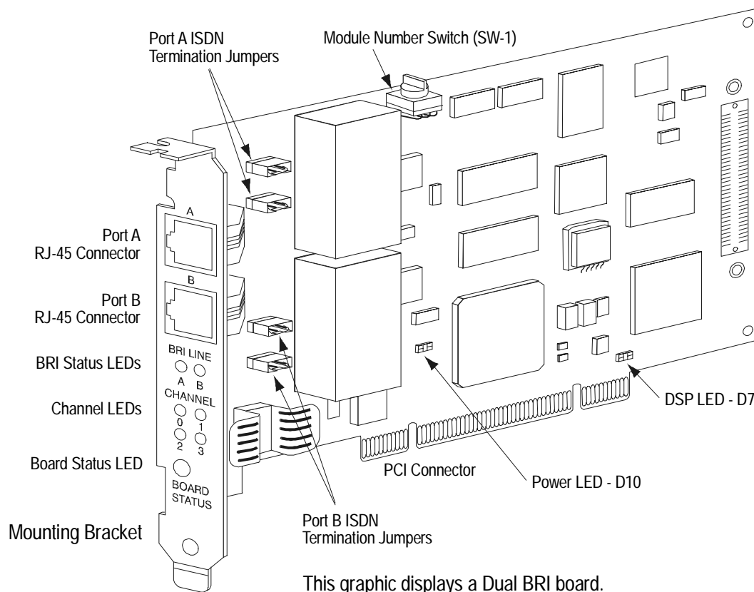
Figure 5. TR1034 BRI PCI Series Board
